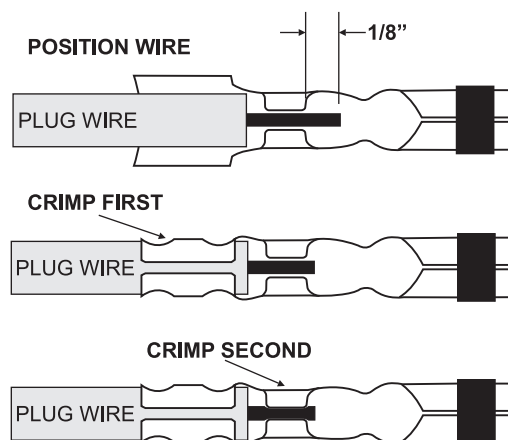
Figure 2 Crimping a Dual Crimp Terminal.
